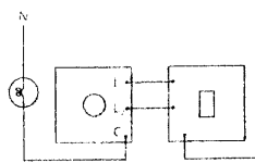
2-Way dimmer connection
