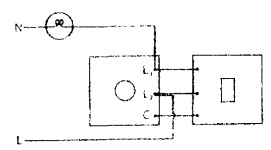
Alternative 2-Way dimmer connection
